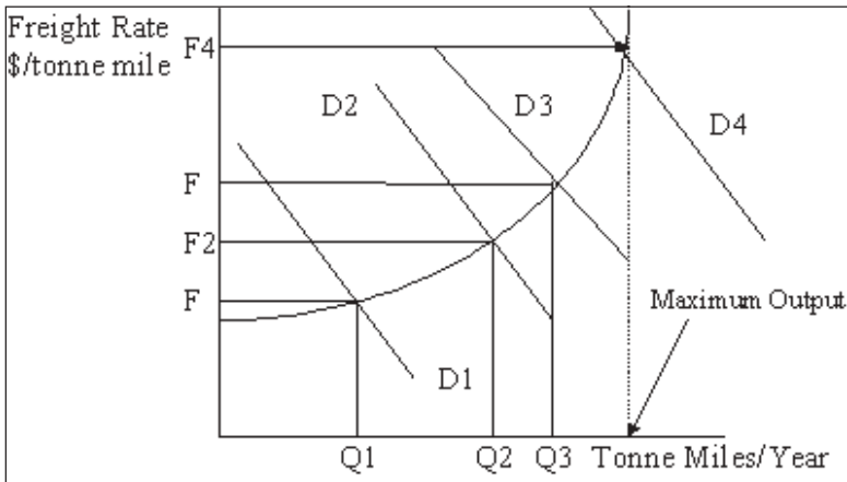
Figure 3 Short Run Market Interaction
