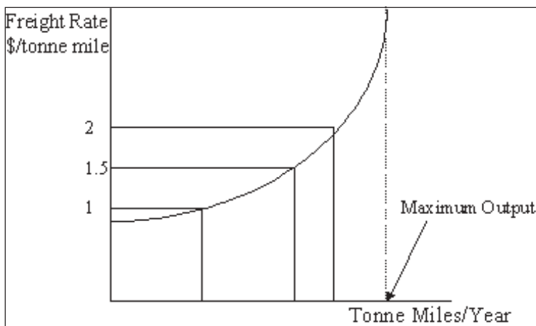
Figure 2 Short Run Shipping Supply Curve
